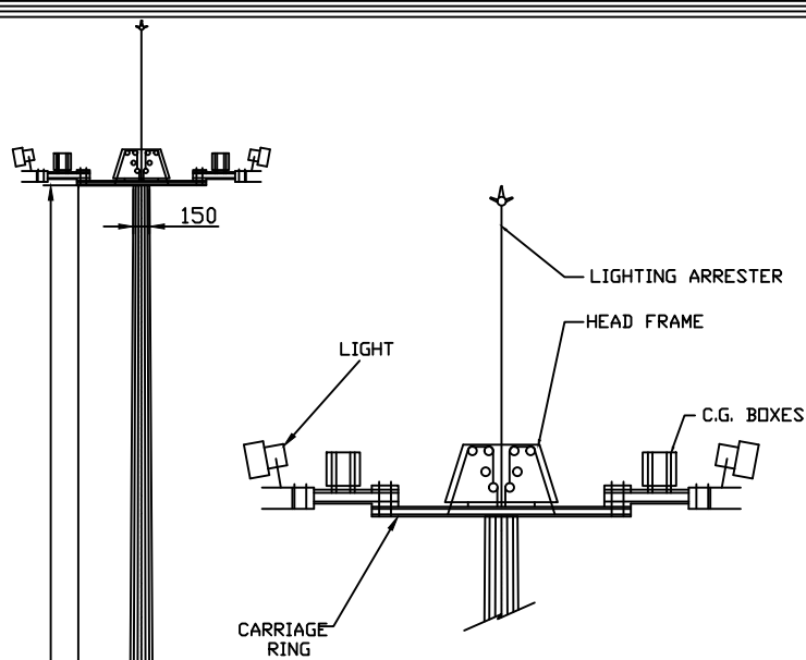
DISTRIBUTION OF LUMINARIES
