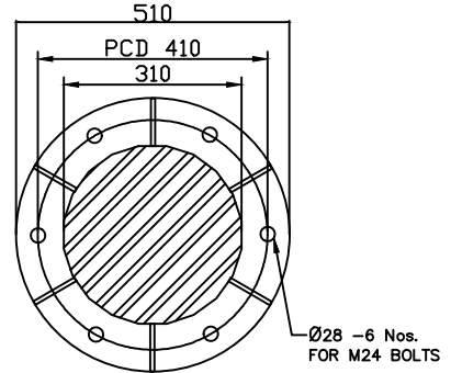
BASE PLATE DIA 510X20 MM THK.
