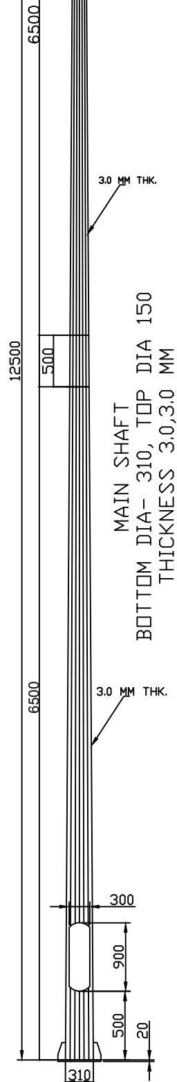
12.5 MTR HIGH MAST POLE WITH 6 LUMINAARIES
